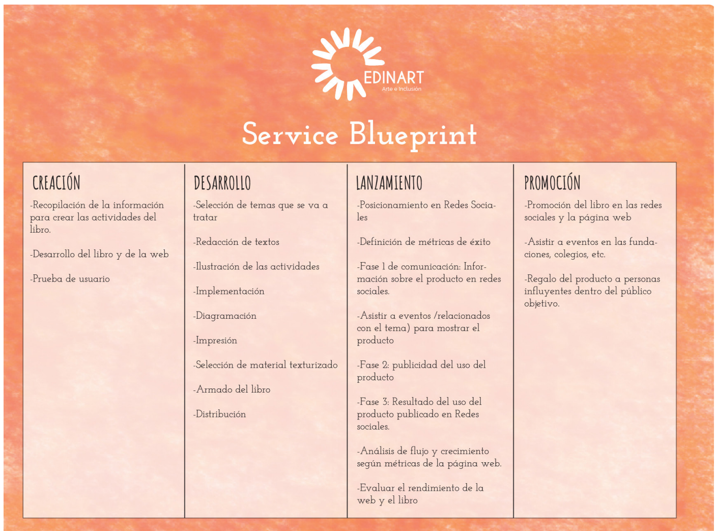
Figura 31: Service Blueprint
